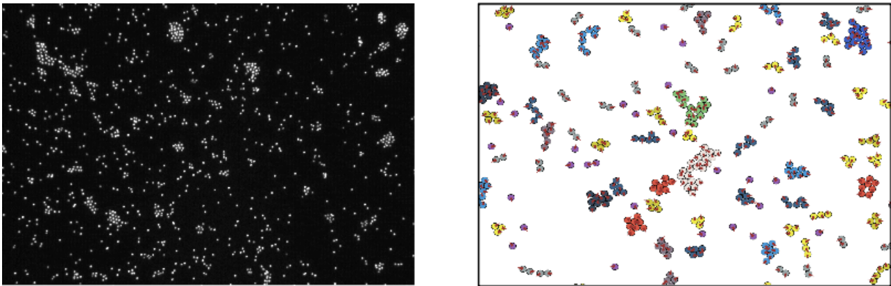
Figure: (Left) Active clusters of active colloids observed in experiments. (Right) Simulation of a minimal model.
