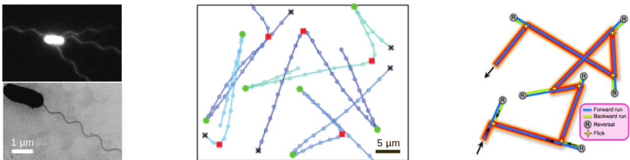
Figure: (Left) Bacteria self-propel by rotating one or several flagella. (Center and Right) Experimentally observed trajectories and schematized swimming pattern. From Son et al, Nature Physics (2013).
