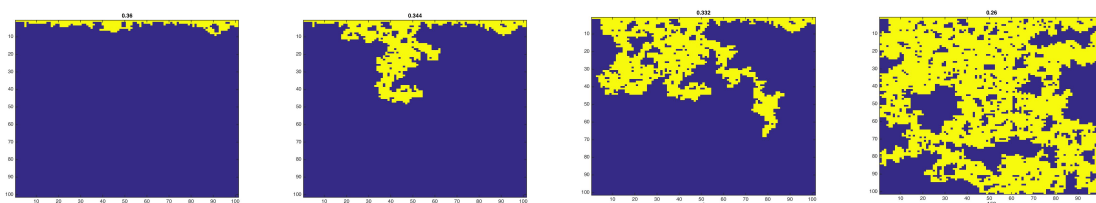
Development of gas phase clusters (yellow) at the expense of the liquid phase (blue) during evaporation in a disordered network of pores. Preliminary simulation in a 2D situation mimicking experimental conditions.
